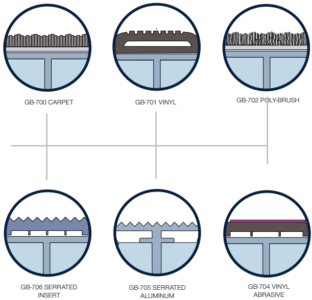
Recessed application includes optional 2" x 2" x 1/4" aluminum frame.
