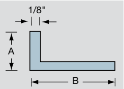
L Series frame available for Recessed Application
