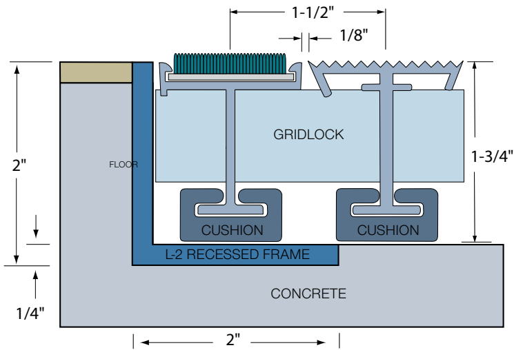
Recessed application includes optional 2" x 2" x 1/4" aluminum frame.
